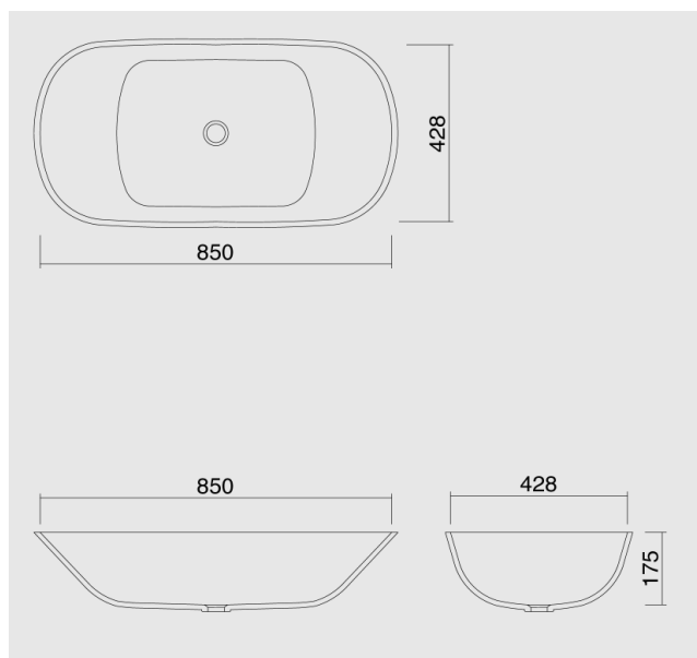
FONTANA FS-68B, double-sided 850 x 428 x 175 mm
